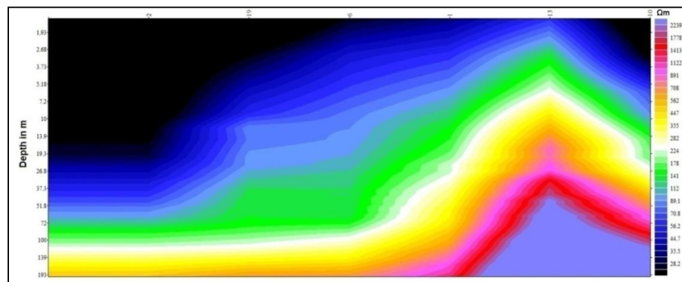
Fig-5: pseudo section of VES-3
