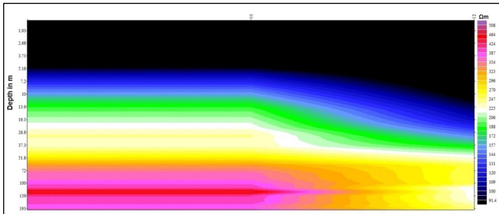
Fig-3: pseudo section of VES-1
