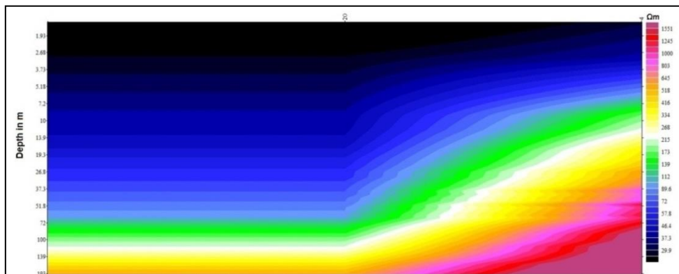
Fig-6: pseudo section of VES-4
