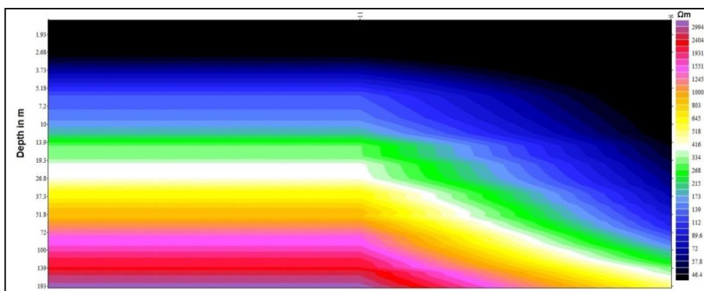
Fig-4: pseudo section of VES-2
