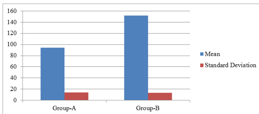
Fig-2: Comparison of Duration of Sensory Block Z=20.88, p<0.05
