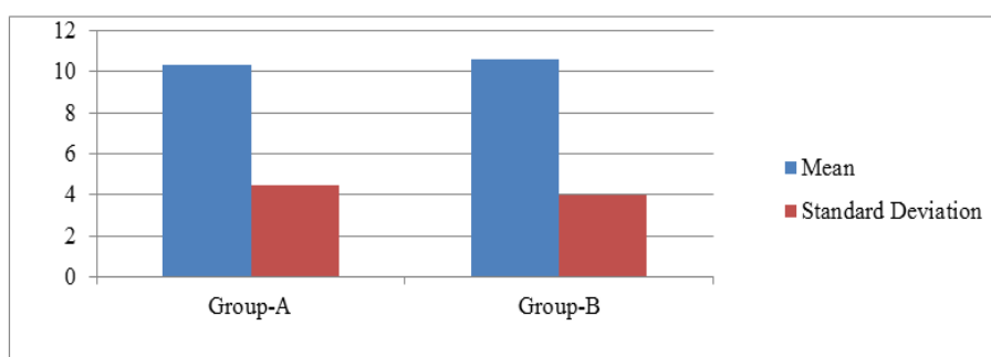
Fig-1: Comparison of Onset of Sensory Block Z=0.28,p>0.05
