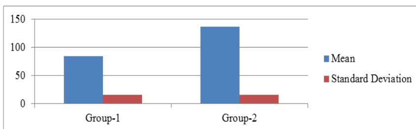
Fig-3: Comparison of Duration of Analgesia Z=16.24, p<0.05
