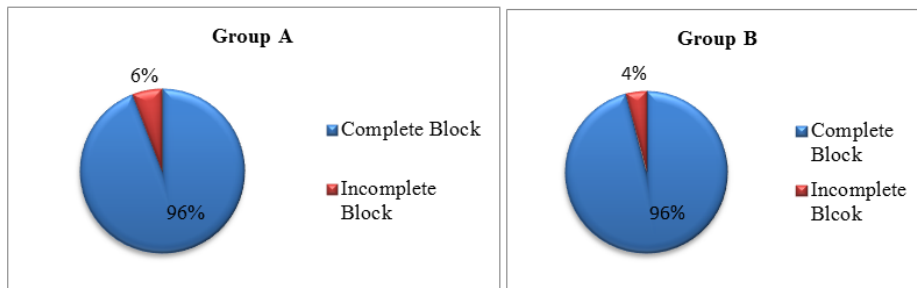
Fig-4: Comparison of Intensity of Motor Block (z=0.465) (p>0.05)
