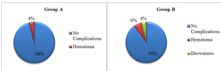
Fig-5: Incidence of Complications
