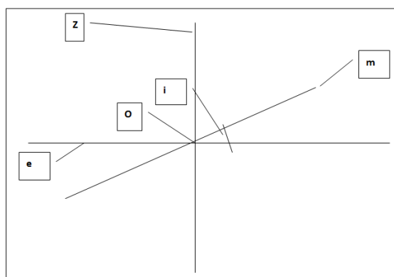
Fig-2: Lateral projection of gravity and orbital planes
