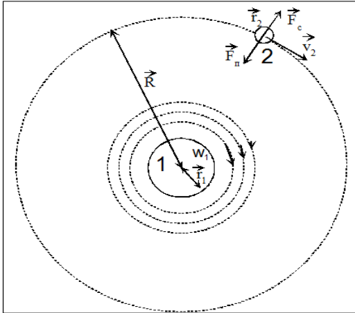
Fig-1: Two-dimensional model of the gravitational interaction of two bodies. The forces acting on the body 2
