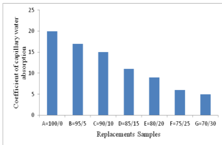
Fig. 3: Coefficient of capillary water absorption for Cement/WGP Composite
