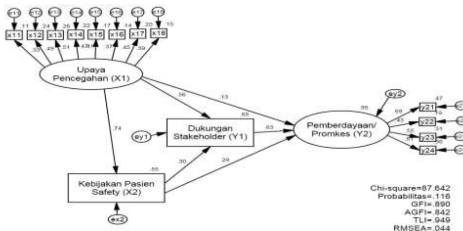
Fig-1: Regression analysis model using determined variables with SEM analysis
