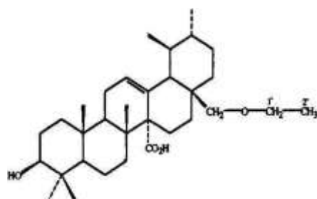
Obtusilinic acid
