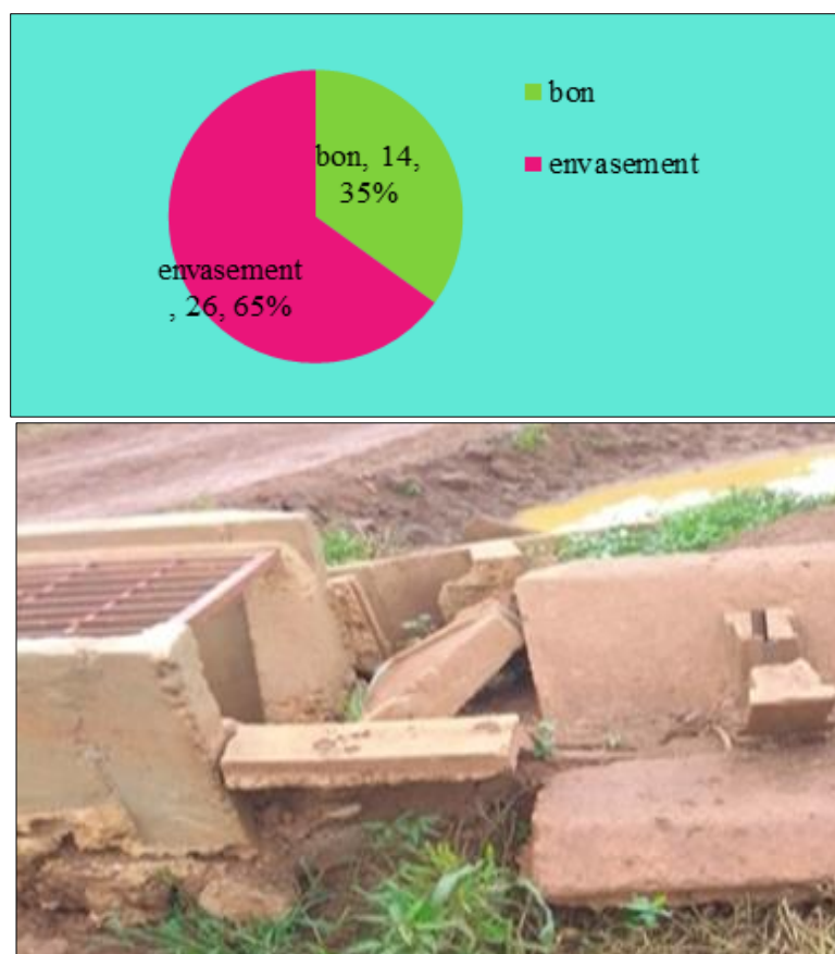
Figure 1 : state of intake structures on the Aneker irrigated perimeter (Source : YERIMA., 2022)
