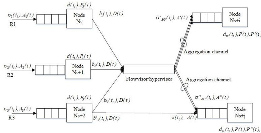
Fig-3: Structural scheme of data provision in NFVI
