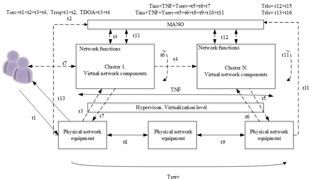
Fig-1: Diagram of service orchestration and provision
