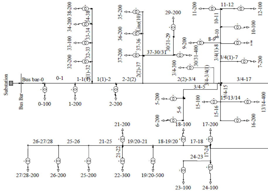
Fig-1: Simulation of Koteswori Feeder in DigSILENT PowerFactory
