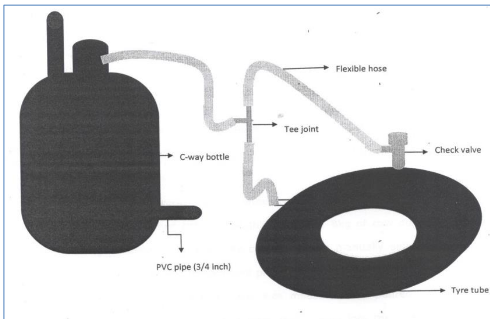
Fig-1: Laboratory Digestion Set-Up
